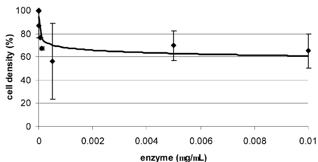
Figure 5. The effect of different concentrations of PGA on the cytotoxicity level of prodrug 7. Human embryonal kidney 293T cells were incubated with 0.5 \mu M prodrug (IC 50 values were calculated as shown in Fig. 4A) and the indicated concentration of PGA. Cell density was measured as in Figure 4A.
